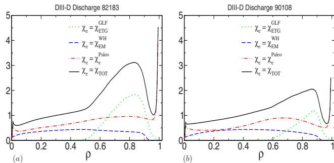
FIG. 9. (Color online) Total electron thermal diffusivity profile and its components computed using model 5 for DIII-D discharge 82183 (left panel) and 90108 (right panel).
