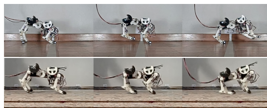
Figure 1: Active (top) and fixed (bottom) spine locomotion.
