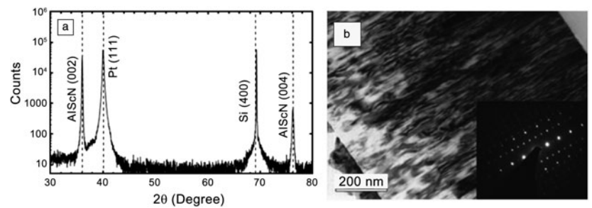
Figure 9. Microstructural analysis of an \text{Al}_{0.88}\text{Sc}_{0.12}\text{N} thin film grown on a Pt (111) bottom electrode at 300°C: (a) \theta –2 \theta x-ray diffractogram; (b) transmission electron microscopy cross-section with the corresponding electron diffraction pattern in the inset (from Reference 57). Note: \theta , angle between the incident x-ray beam and the incident plane.
