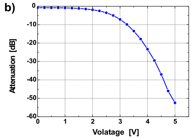
Fig. 4. a) The variable optical attenuator (VOA) moves a shutter in between two fibers. B) The attenuation of the VOA has a dynamic range of over 50 dB.
