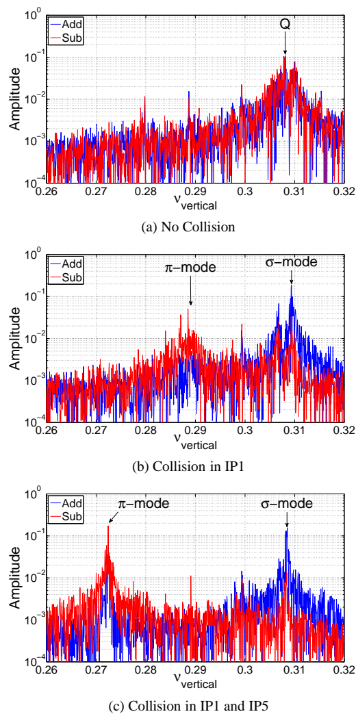
Figure 2: The Fourier transform of the addition and subtraction of the beam position measured by the BBQ pickups.
