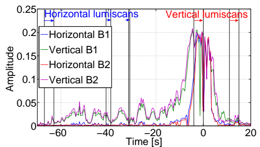
(a) Amplitude of the BBQ signal
