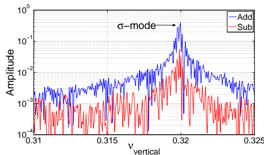
(b) Spectrum at t = -10 s
