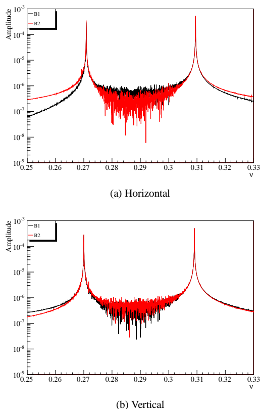
Figure 1: Simulation of coherent spectrum for the experiment 1. A tune shift of \Delta Q_{\text{sim}} = 0.040 is observed between the two coherent modes.
