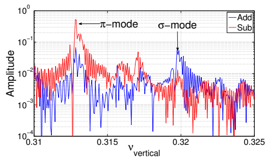
(c) Spectrum at t = 1 s
