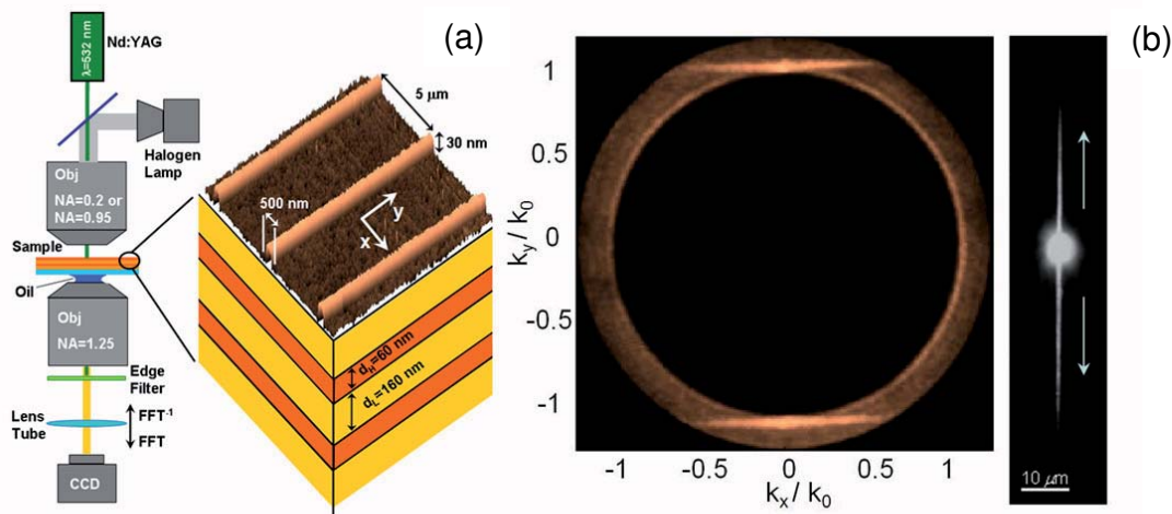
(a) LRM setup for detecting fluorescent GBSW on nanometric ridges (AFM map on multilayer sketch); (b) Fourier and direct plane images of fluorescent GBSW on single guide.
