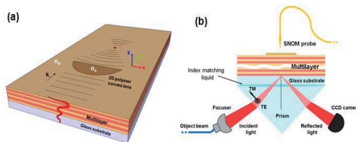
Fig 1. (a) Concept of the 2D plano-convex lens. The field is confined at the surface of the multilayer. An ultra thin convex lens made of AZ1518 is coated on top of the platform; (b) BSWs excitation is performed in the Kretschmann configuration using a BK7-glass prism.
