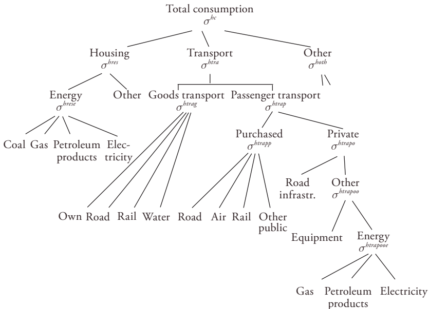
Figure 3: Structure of the Households' Nested CES Utility Function
