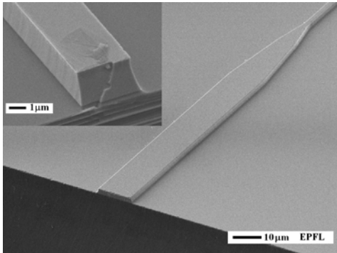
Figure 3 : SEM image of the waveguide. The coupling part is 15 μm wide and the narrower part is 2.9 μm wide. The in-set is the cross-section in the straight section. [11].
