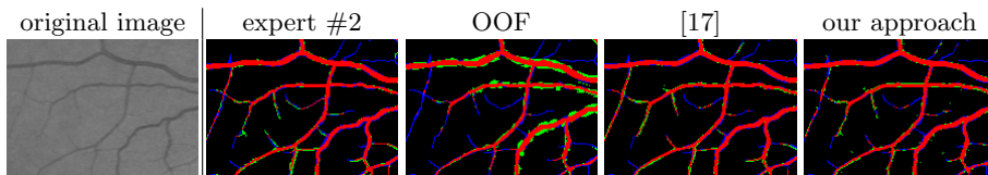
Fig. 3. Qualitative segmentation results on a randomly selected part of an image randomly chosen from the DRIVE dataset. True positives are outlined in red, false positives in green, and false negatives in blue. The segmentation accuracies for [17] and our approach are comparable, while our approach is much more efficient.
