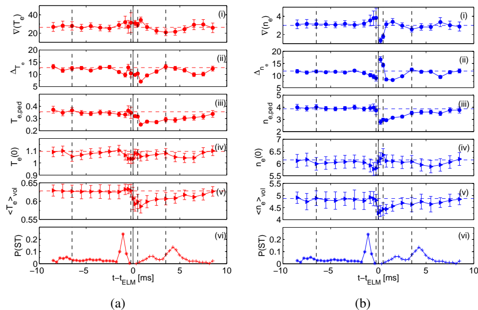
Figure 1: Time evolution of profile parameters during cycles with type-III ELMs (a) temperature, (b) density, (i) max. gradient, (ii) pedestal width, (iii) pedestal height, (iv) centre value, (v) vol.-averaged value, (vi) probability for sawtooth event
