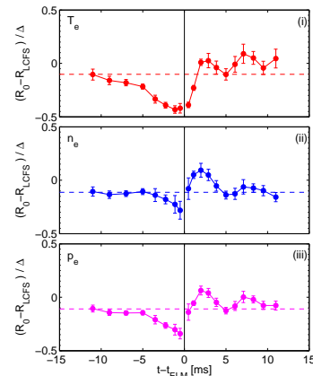
Figure 4: Displacement of edge barrier with respect to separatrix for type-I ELMs
