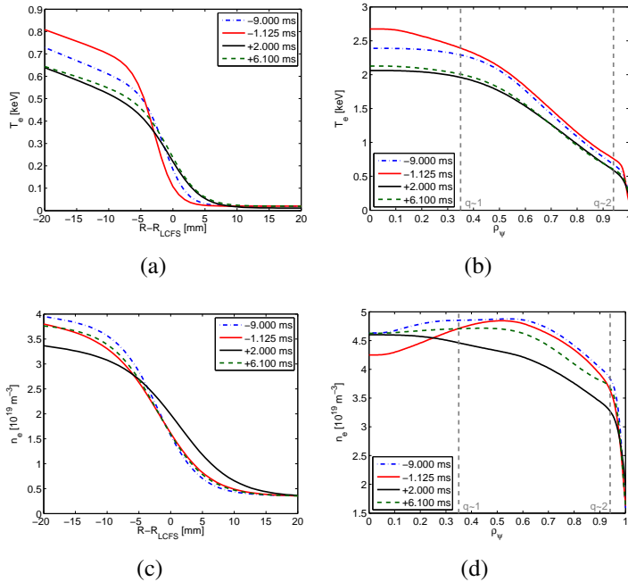
Figure 3: Profiles of T_e and n_e at selected times during a cycle with type-I ELMs
