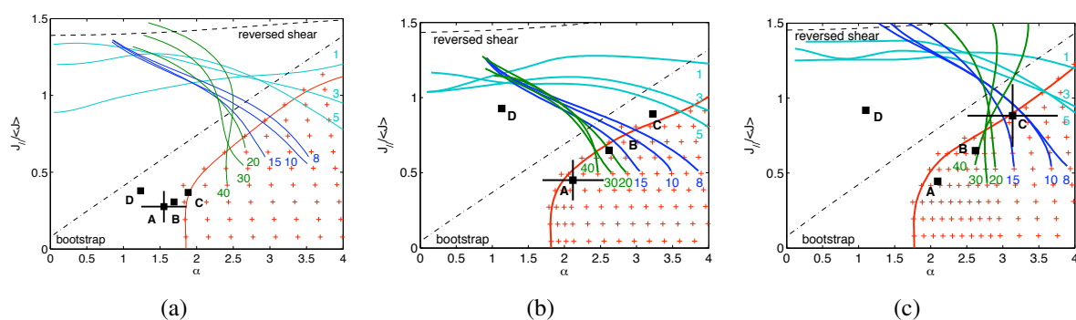
Figure 5: Stability diagram for the plasma edge from ideal MHD calculations
