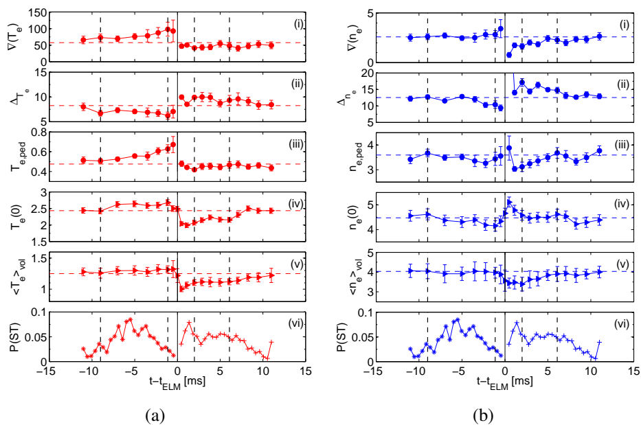
Figure 2: Time evolution of profile parameters during cycles with type-I ELMs same identification as in fig. 1
