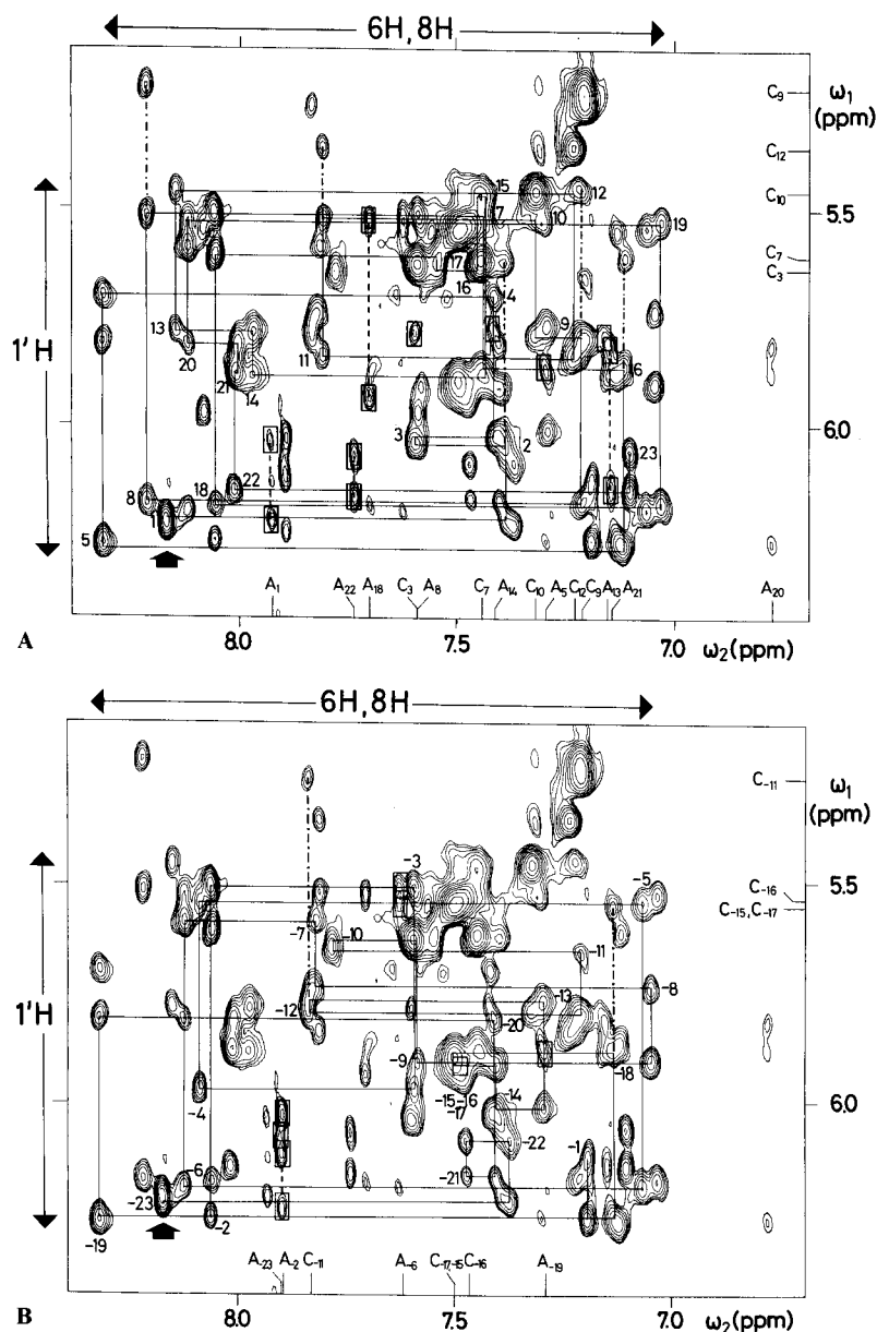
Fig. 2A and B. Region of the 500 MHz absorption mode NOESY spectrum of the 23-bp DNA of Fig. 3 recorded with 100 ms mixing time, showing the sequential connectivities d_i(6, 8; 1') followed by d_s(1'; 6, 8) for the (+)-strand (A) and the (-)-strand (B), respectively. Intra-residue cross peaks are labeled with the nucleotide number. Cross peaks between A2H and 1'H are labeled with frames and connected by broken lines if they involve the same A2H. Cross peaks due to d_s(6, 8; 5) are connected to either the cross peaks d_i(6, 8; 1') or d_s(1'; 6, 8) of the same 6 or 8 proton by dashed-dotted vertical lines. The resonance positions of the A2H's are indicated at the bottom of the figure. The strong cross peaks d_i(5; 6) of the cytosines are identified at the right side for the 5H and at the bottom for the 6H. The start of the assignment pathway at the 5' end is indicated by an arrow
