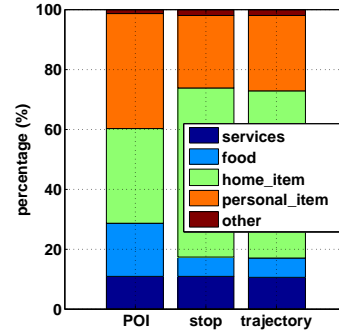
Fig. 27: Semantic stops/trajectories by HMM-based POI annotation
