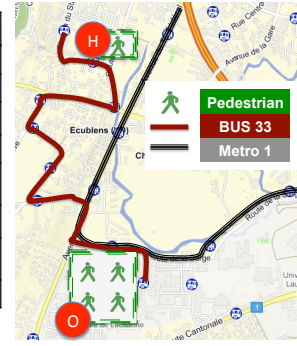
Fig. 30: Ground truth
