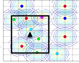
Fig. 17: Discretization
