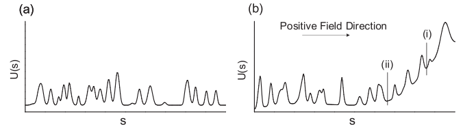
FIG. 4. Schematics of energy functions U(s) for domain wall displacements, s . (a) Position of a domain wall, with random potentials and without asymmetry. (b) Position of a domain wall after a strong electric field is applied towards the right-hand side (positive) in (i); deaged position of a domain wall in (ii).
