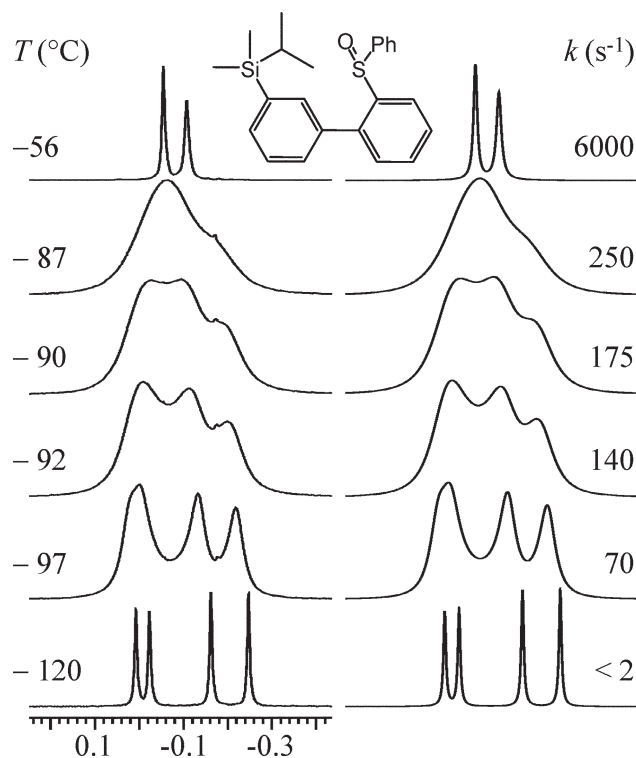
Fig. 2 Left: temperature dependence of the silicon bonded ^1\text{H} NMR methyl signals of ortho phenyl sulfoxide derivative 3 in \text{CHF}_2\text{Cl}/\text{CHFCl}_2 at 600 MHz. Right: line shape simulation obtained with the indicated rate constants.
