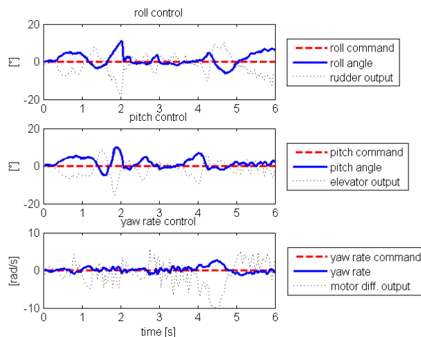
Fig. 6. Example attitude stabilization in hover mode, where the pitch and roll angles and the yaw rate are automatically stabilized around zero.
