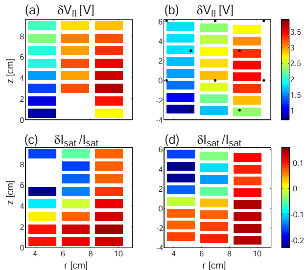
FIG. 5. (color online) (a), (c) : Effects on V_{fl} and I_{sat} profiles due to the biasing, measured directly on the limiter. The square white area corresponds to the position of the electrodes that are used for the biasing. (b), (d): The same measurements, but obtained with HEXTIP, at 90^\circ from the limiter. Measurements at the positions indicated by black dots in (b) are linearly interpolated to obtain the values on the flux tubes connected to each electrode.
