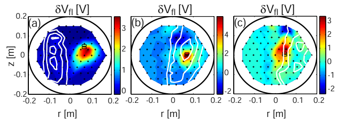
FIG. 6. (color online) \delta V_{fl} for plasmas with reversed field ( B_\phi, B_z < 0 ) and B_\phi = -75.6 mT (a), -86.4 mT (b), and -91.0 mT (c). I_{sat} profiles are indicated by white contours.
