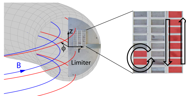
FIG. 1. (color online) Sketch of the TORPEX vacuum vessel and the electrodes installed on a conducting limiter. Examples of magnetic field lines and the coordinate system are also shown. A zoomed view of the electrodes is shown at the right. Shaded areas indicate examples of positively biased electrodes and arrows show the expected flow pattern.
