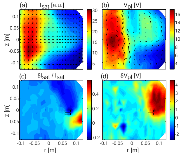
FIG. 2. (color online) Profiles of (a) I_{sat} and (b) V_{pl} measured with SLP. Measurement points are indicated by the +’s in (a). Vectors in (b) represent the \mathbf{E} \times \mathbf{B} velocity. (c) and (d) show the relative changes in I_{sat} and the absolute changes in V_{pl} induced by biasing the indicated set of electrodes to +40 \text{ V} .
