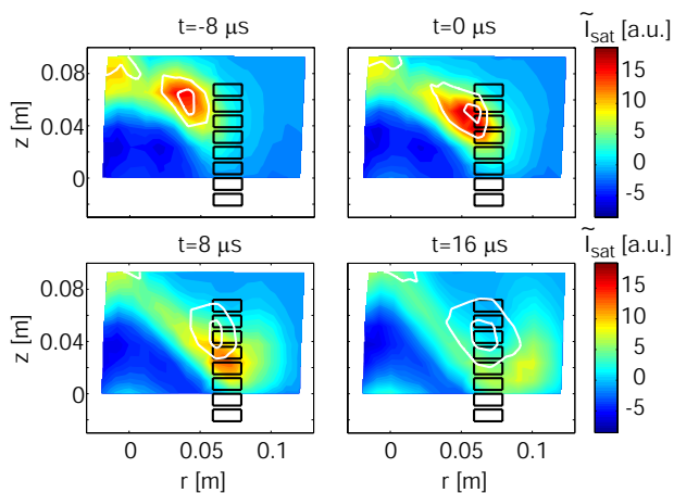
FIG. 3. (color online) Conditionally averaged blob propagation ( I_{sat} fluctuations) for the case where a vertical stripe of electrodes is biased to +40 V (color plots). For comparison, the white contours indicate the results of the same analysis when all electrodes are grounded.
