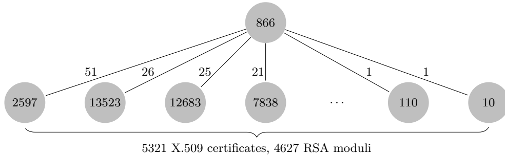
Fig. 4. The largest depth one tree found, on 4628 vertices, with the 512-bit prime p_{866} as root and leaves p_{2597}, p_{13523}, \dots, p_{10} . The edges correspond to 4627 distinct 1024-bit RSA moduli, with labels indicating the number of distinct X.509 certificates and PGP keys containing the RSA modulus corresponding to the edge, for a total of 5321 certificates. All certificates have expired and use SHA1 as hash function.
