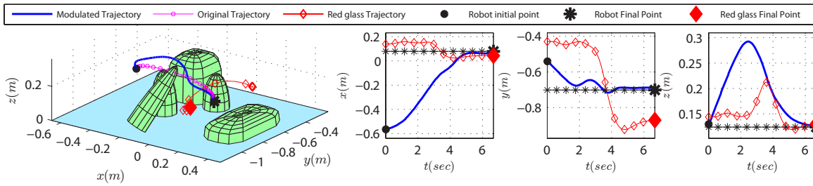
(b) Illustration of the robot, target and obstacle motions for the first trial.
