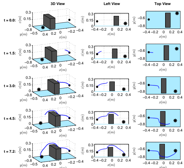
(c) Illustration of the sequences of the motion
