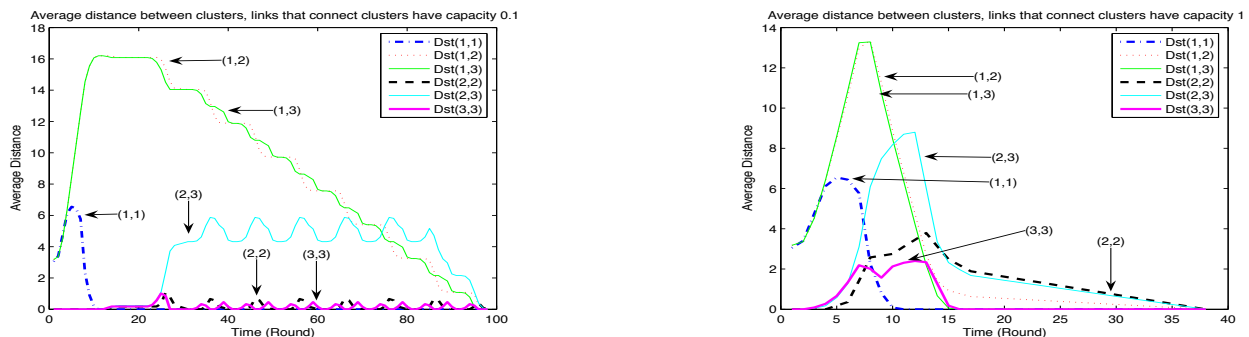
Fig. 8. Simulation results for the topology in Figure 7, with bottleneck link capacity values equal to 0.1 (left) and 1 (right).
