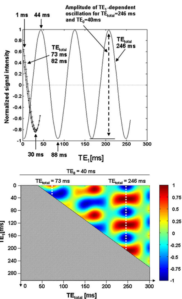
Fig. 1. Upper panel: Citrate signal intensity oscillations (intensity of the fully refocused multiplet normalized to 1) as a function of TE_1 while TE_{total} and TE_0 (40 ms) remain fixed. TE_2 is determined by TE_2 = TE_{total} - TE_0 - TE_1 . The citrate signal oscillates between a positively (up) and a negatively (down) refocused lineshape, as indicated for TE_{total} = 246 ms, 73 ms or 82 ms. The oscillation amplitude strongly depends on the choice of TE_{total} and TE_0 (see Fig. 2). Lower panel: Simulated citrate signal intensity (3rd dimension) as a function of the total echo time ( TE_{total} , x-axis) and TE_1 (y-axis) using 3S-PRESS. TE_0 was fixed to 40 ms and impossible combinations of TE_{total} and TE_1 were excluded from the plot. Vertical cuts as indicated for TE_{total} = 246 ms (compare to upper panel) and TE_{total} = 73 ms represent the TE_1 dependent oscillations at fixed TE_{total} which are used for editing.
