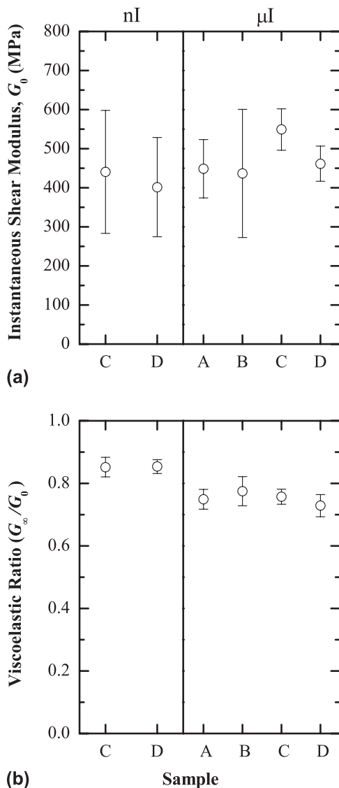
FIG. 3. Instantaneous shear modulus ( G_0 ) and viscoelastic ratio ( G_\infty/G_0 ) for bone specimens tested by nanoindentation (nI) or microindentation (μI). The elastic moduli did not vary, but there was a slight difference in viscoelastic ratio.
