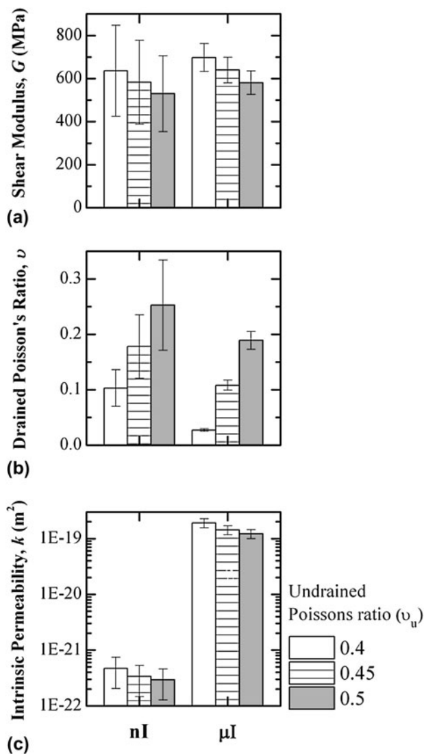
FIG. 5. Poroelastic parameters identified from spherical nanoindentation and microindentation tests on a single bone specimen. The undrained Poisson's ratio ( \nu_u ) was assigned a value of 0.4, 0.45 or 0.5 to assess sensitivity of the parameter identification process on this value.
