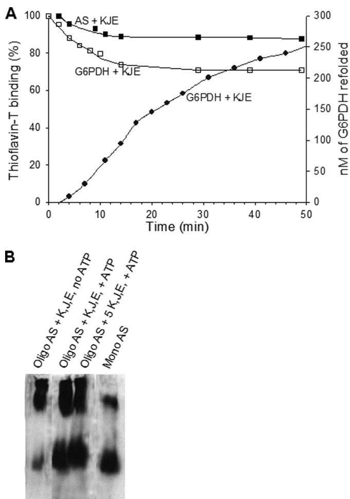
FIGURE 4. AS oligomers are partially resistant to the Hsp70 chaperone machinery. A , AS oligomers are more resistant to the unfolding chaperones than G6PDH aggregates. Time-dependent loss of Th-T fluorescence ( squares ) of 1 \mu M heat pre-aggregated G6PDH ( open squares ) or 1 \mu M (protomers) AS oligomers ( filled squares ) in the presence of 5 \mu M DnaK, 0.75 \mu M DnaJ, and 1 \mu M GrpE ( KJE ) and ATP and the corresponding time-dependent reactivation of native G6PDH ( filled circles ) is shown. B , AS oligomers are partially dissociated by the ATP-fueled DnaK/DnaJ/GrpE chaperone system. AS oligomers were incubated as in A but for 3 h at 30°C with or without ATP and chaperones, as specified. Samples were separated on native gel, and \alpha -synuclein was detected by Western blot analysis as in Fig. 1.
