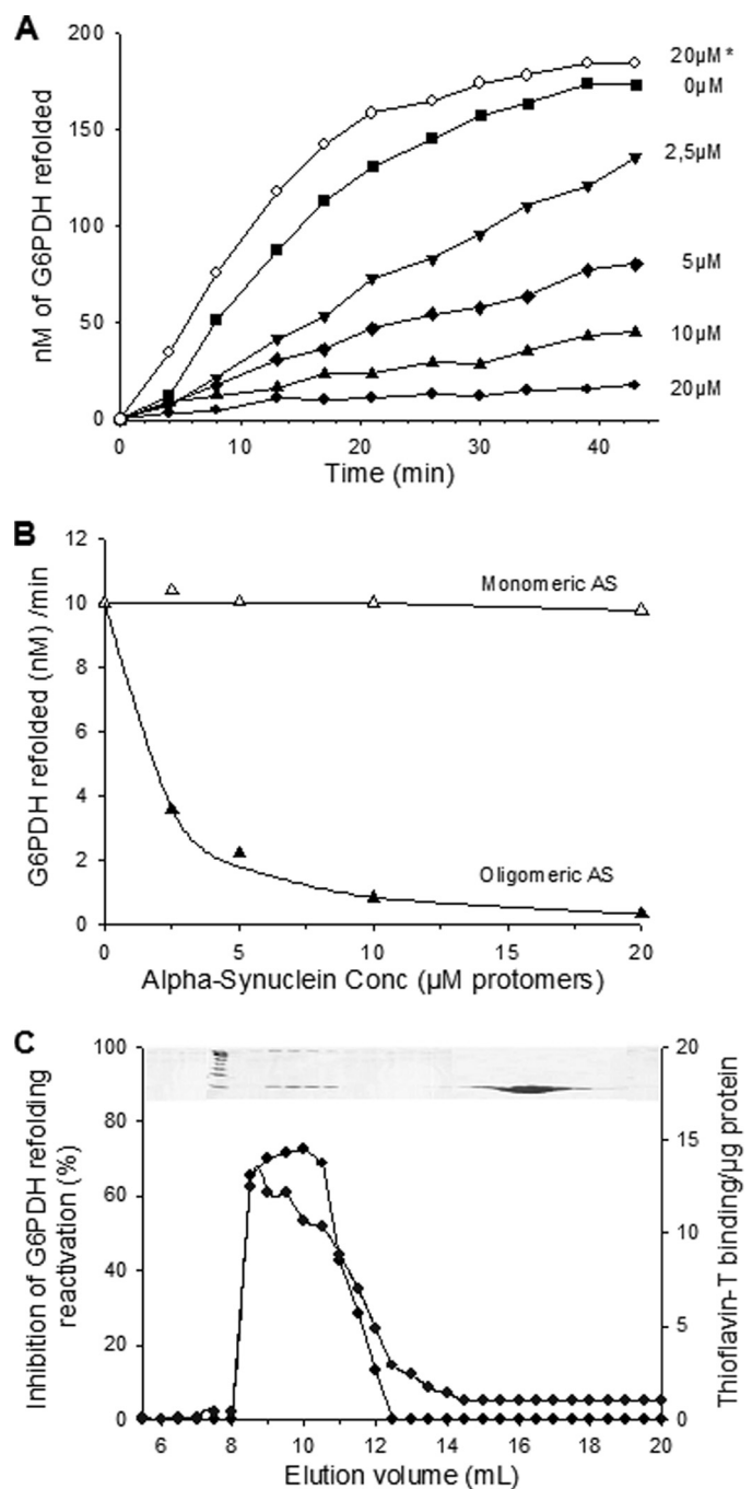
FIGURE 5. AS oligomers inhibit the unfolding/refolding activity of the Hsp70 chaperone system. A , time-dependent reactivation of heat-pre-aggregated G6PDH by the full DnaK chaperone system is shown. The heat pre-aggregated G6PDH (0.75 \mu M) was first incubated with increasing concentrations of AS oligomers (0–20 \mu M protomers) ( filled symbols ) or 20 \mu M AS monomers ( open symbols, asterisk ) and then incubated with 5 \mu M DnaK, 1 \mu M DnaJ, 0.5 \mu M GrpE, and ATP. B , optimal G6PDH refolding rates from A as a function of increasing concentrations of AS monomers ( open triangles ) or oligomers ( filled triangles ) are shown. C , the specific chaperone inhibitory activity profile ( open circles ) compared with the Th-T binding profile ( filled circles ) of AS species in the different fractions from the size exclusion chromatography in Fig. 2 B is shown.
