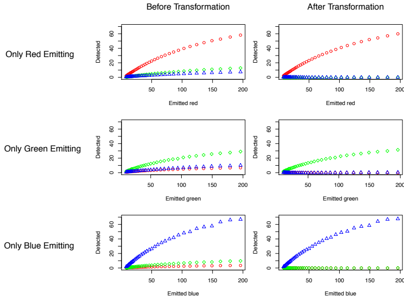
Fig. 11 Each one of the three components of colour detected by the omni-directional camera, before and after transformation.
