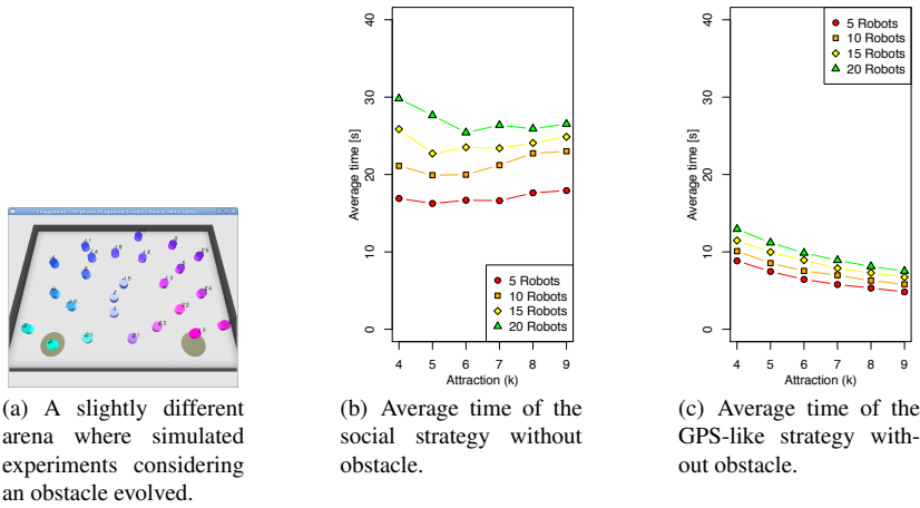
Fig. 5 a) Tag 1 is placed in the bottom-left corner, and tag 2 is placed in the bottom-right corner. b) and c) Average time a searching robot spends in going from one target to the other without the presence of obstacles in the environment. Different values of k and different amounts of robots searching for targets at the same time were tested.
