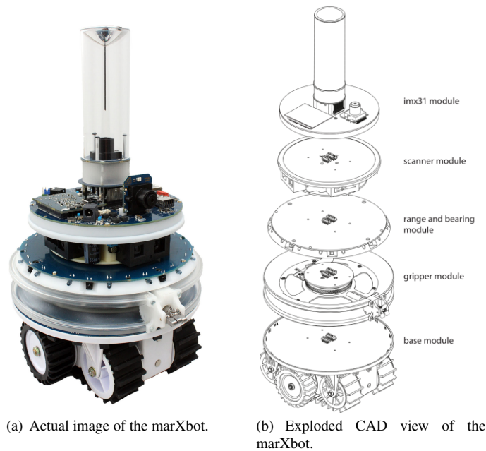
Fig. 9 The marXbot in a configuration including five modules.
