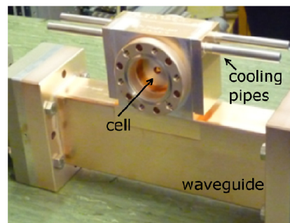
Figure 3: 3 GHz single-cell cavity.
