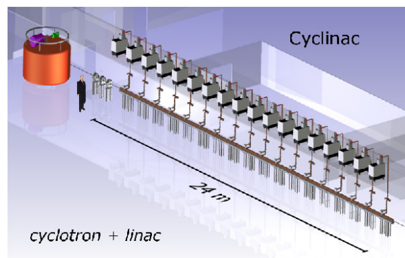
Figure 1: Cyclinac complex for hadrontherapy [2].
