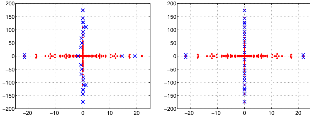
Fig. 1 Eigenvalues (‘.’) and approximate eigenvalues (‘x’) computed by a standard Arnoldi method (left picture) and by a structure-preserving Arnoldi method (right picture).
