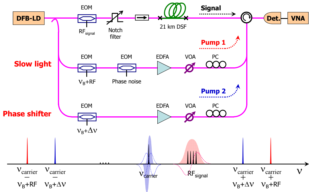
Figure 9. Top: Diagram of the experimental setup realizing true time delays using the separate carrier tuning technique. The true time delaying on the optical sideband is realized using a Brillouin slow light system with a spectrally broadened pump 7 to cover the bandwidth of the microwave modulation. The phase shifting is implemented using the system described in Section 2. All optical signals (pumps and optical carrier) are generated from the same laser source. Bottom: Graphical representation of all optical signals present in the system, with the 3 combined Brillouin interactions.
