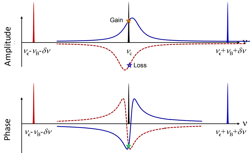
Figure 5. Principle of the phase shifting function realized using stimulated Brillouin scattering in optical fibers. Two optical monochromatic pumps are symmetrically placed at a frequency close to the Brillouin resonance frequency \nu_B below and above the signal frequency, respectively. If the 2 pumps are slightly but equally detuned by \delta\nu with respect to the peak central resonance frequency, the generated gain and loss exactly compensate while the phase changes sum up.
