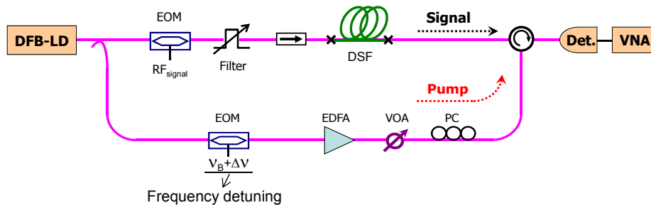
Figure 6. Schematic diagram of a microwave phase shifter realized using the principle depicted in Figure 5 in an optical fiber. The 2 pumps for the Brillouin interaction are generated from the same laser source modulated by the microwave signal, in a distinct fiber channel using an electro-optic modulator. EOM: electro-optic modulator, EDFA: erbium doped fiber amplifier, VOA: variable optical attenuator, DSF: dispersion-shifted fiber, VNA: vector network analyzer.
