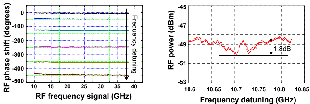
Figure 7. Left: Phase shifts obtained for different microwave carrier frequency between 10 and 40 GHz, showing the total absence of dependence on the frequency. The phase shifts cover a range exceeding 400^\circ . Right: amplitude change of the microwave signal for different frequency detuning, corresponding to the phase shift range shown on the left graph.
