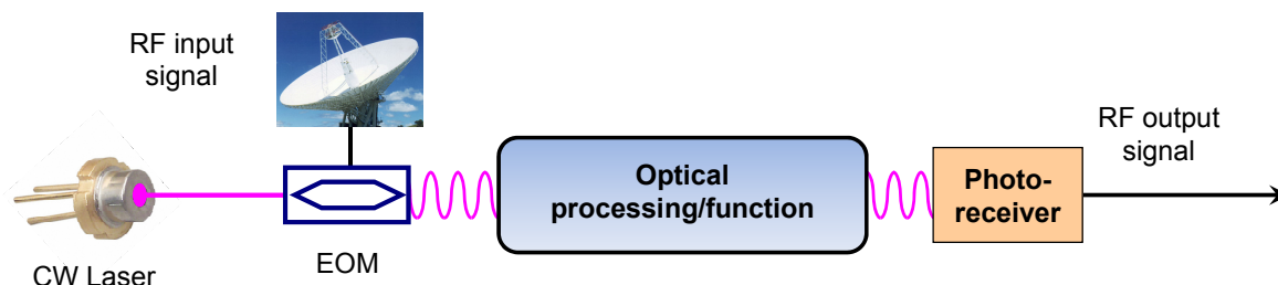
Figure 1. Concept of a microwave photonics system: the microwave signal is converted into the optical domain through an optical modulation, is then transformed using an optical processing/function to eventually return into the electrical domain through a broadband photodetection.
