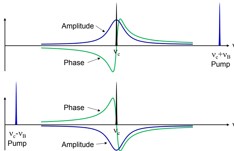
Figure 4. Spectral distribution of the amplitude and phase changes generated by stimulated Brillouin scattering. An optical wave will experience amplification if the medium is pumped by an optical wave at a frequency \nu_B over the signal frequency \nu_c (top graph). The pump must propagate in the direction opposite to the signal. If the pump is spectrally placed at a frequency \nu_B below the signal frequency \nu_c , the signal will be attenuated (bottom graph). The phase shift is zero at the center of the resonance, but follows a linear relationship for small frequency detuning.
