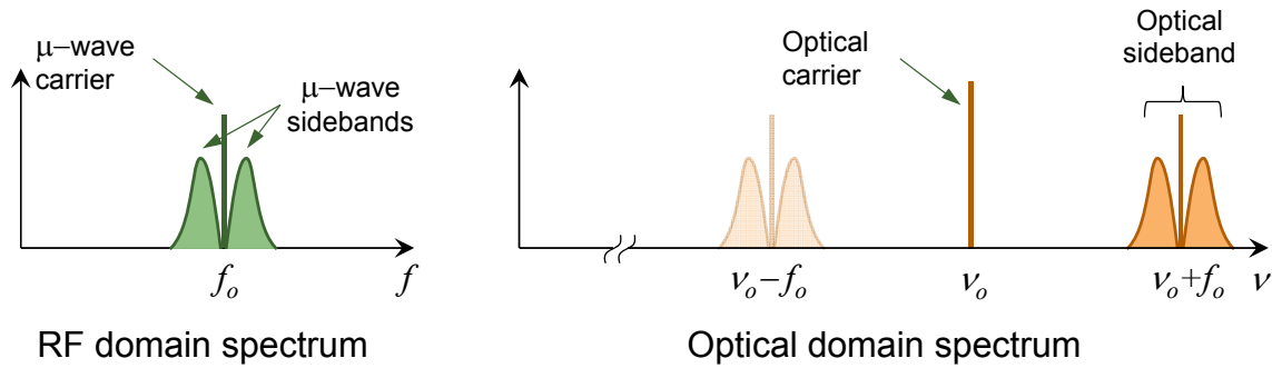
Figure 2. Spectral contents of the microwave (left) and optical (right) signals, respectively. The entire spectral content of the microwave signal is contained in the optical sidebands, separated from the optical carrier by the microwave carrier frequency. One of the optical sidebands is generally suppressed without any loss of information.
