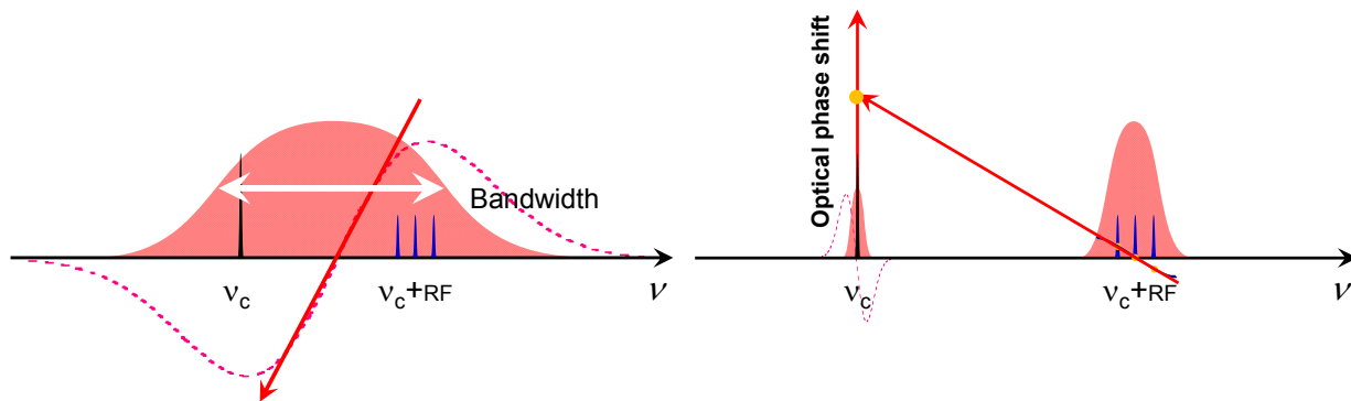
Figure 8. Left: Direct true time delaying using a slow light interaction covering the full bandwidth occupied by the optical signal. A wide spectral range covered by the interaction contains no spectral information. Right: True time delaying realized using the separate carrier tuning technique. The interaction covers only the optical sideband and the phase of the carrier is separately adjusted to match the linear frequency dependence of the phase shifts.
