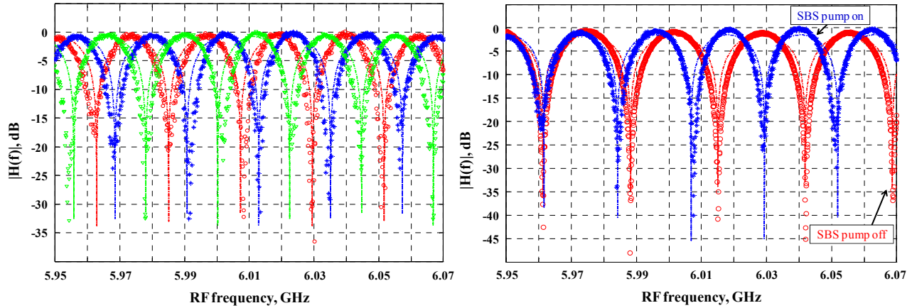
Figure 11. Left: Notch filter response for 3 different phase shifts applied to the optical carrier, showing the possibility to dynamically position a notch at any frequency thanks to the phase shifting capability over more than 360°. Right: Notch filter response with and without true time delaying, demonstrating the possibility to substantially adjust the spectral periodicity of the notch response (20%).
