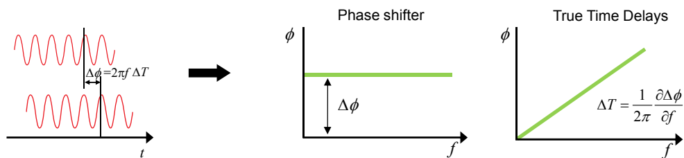
Figure 3. Left: For a single frequency signal phase shift \Delta\phi and time delay \Delta T are closely and unambiguously related. Right: In the case of a signal containing many frequencies, phase shifting and time delaying do not have the same meaning, leading to different functions and resulting to a different dependence of the phase shift on the frequency.
