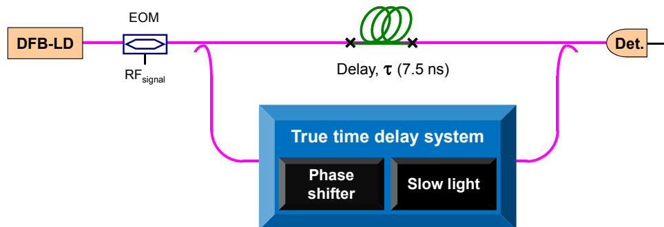
Figure 10. Schematic diagram of a dynamic microwave photonics notch filter. The frequency position of the notches can be tuned with the phase shifter, while the frequency spacing between the notches can be modified by applying a true time delaying in one of the arms.
