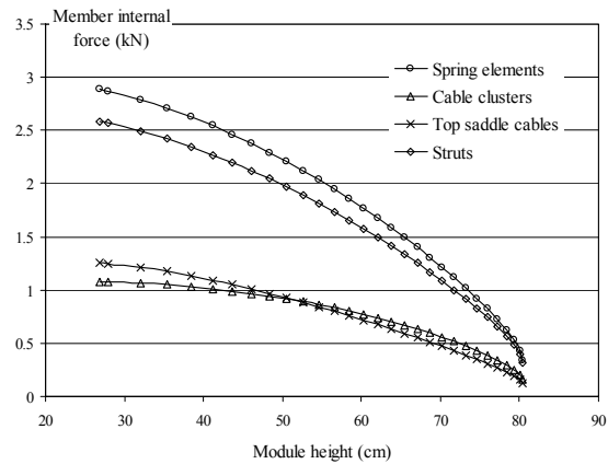
Figure 12. Internal force magnitudes in the tensegrity members during deployment
