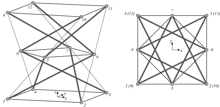
Figure 9. Perspective and top views of the two-module tensegrity structure
