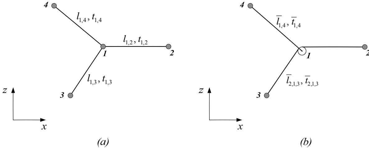
Figure 1. A three-element structure and the equivalent configuration with one continuous cable.
