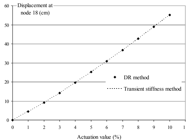
Figure 5. Actuation-response of the clustered tensegrity beam
