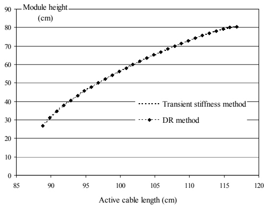
Figure 11. Actuation-response of the clustered tensegrity structure
