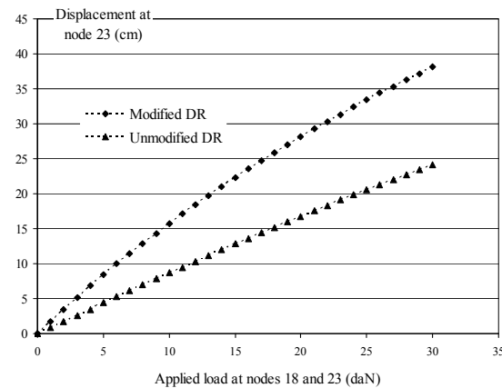
Figure 8. Load-displacement curves obtained employing modified and unmodified DR
