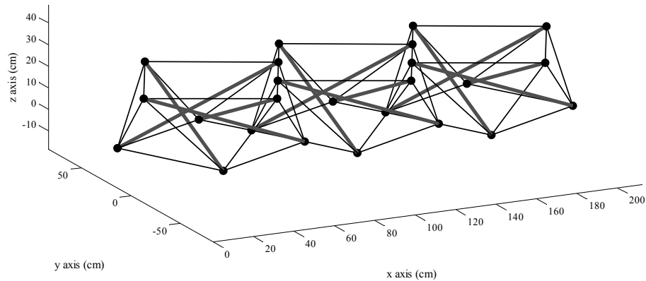
Figure 3. A perspective view of the tensegrity beam
