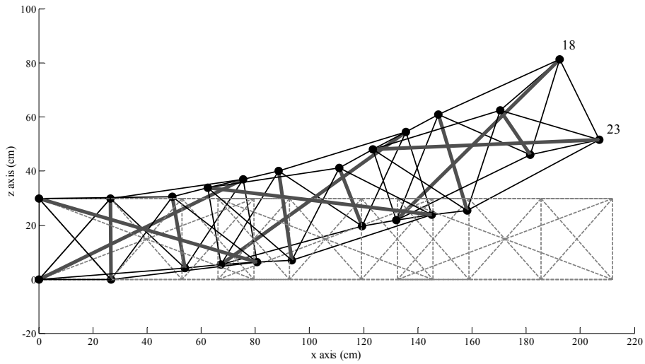
Figure 6. Deformed shape of the tensegrity beam due to 10% actuation of cable clusters
