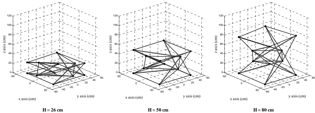
Figure 10. Snapshots of the deployment process of the two-stage tensegrity structure
