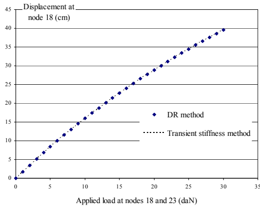
Figure 7. Load-displacement curves of the clustered tensegrity beam
