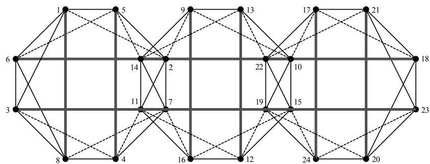
Figure 4. Clustered elements of the tensegrity beam
