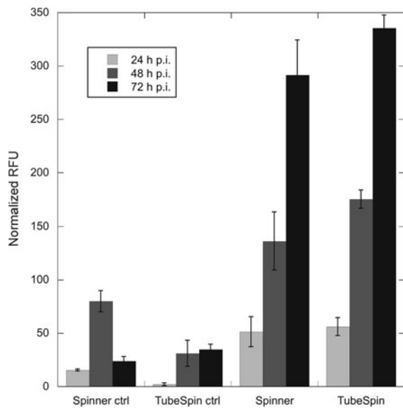
Fig. 4 Comparison of recombinant GFP production in Sf-9 cultures grown in spinner flasks and TubeSpins. The cells at 2 \times 10^6 cells/ml were infected with baculovirus at MOI 2–3 or left uninfected ( ctrl ). The cultures were analyzed for GFP-specific fluorescence at various times post-infection as indicated. For the cultures in spinner flasks, each bar represents the average of two independent experiments, and for the cultures in TubeSpins, each bar represents the average of two independent experiments performed in duplicate
