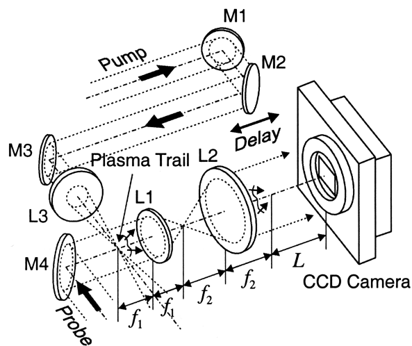
Fig. 1. Holographic setup. An intense femtosecond laser pulse (the pump pulse) is focused by L3 and leaves a plasma trail. A probe pulse traverses the plasma trail a few picoseconds after the pump pulse goes through. The system has a magnification of f_2/f_1 . L1–L3, lenses; M1–M4, mirrors.
