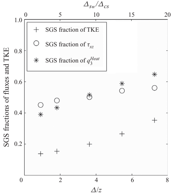
FIGURE 5. SGS fractions of the TKE and of the vertical fluxes of heat ( q_3^{Heat} ) and momentum \tau_{xz} as a function of filter size (lower x-axis) and filter aspect ratio (upper x-axis).
