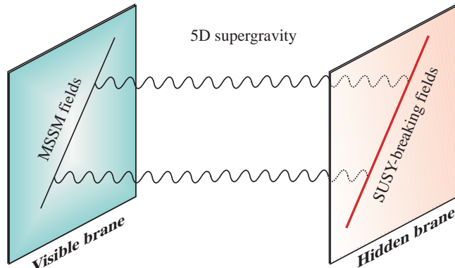
Figure 1: One-loop supergravity diagrams inducing an effective interaction between visible and hidden sector.
