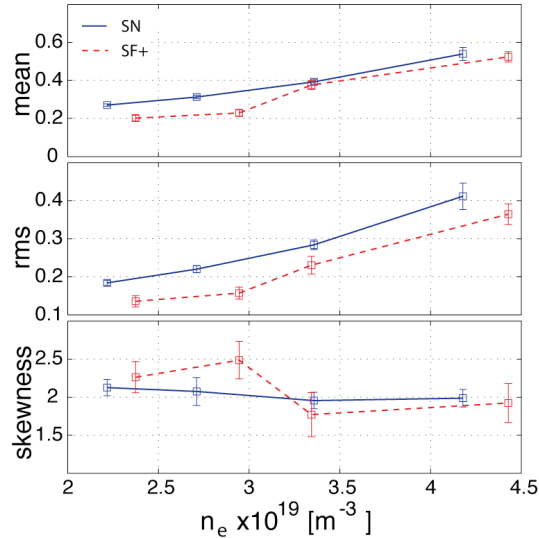
FIG. 5: Moments of the ion saturation current density J_{sat} for different plasma densities for SN (solid) and for SF+ (dashed). Squares correspond to the average value between probes #1-#3.
