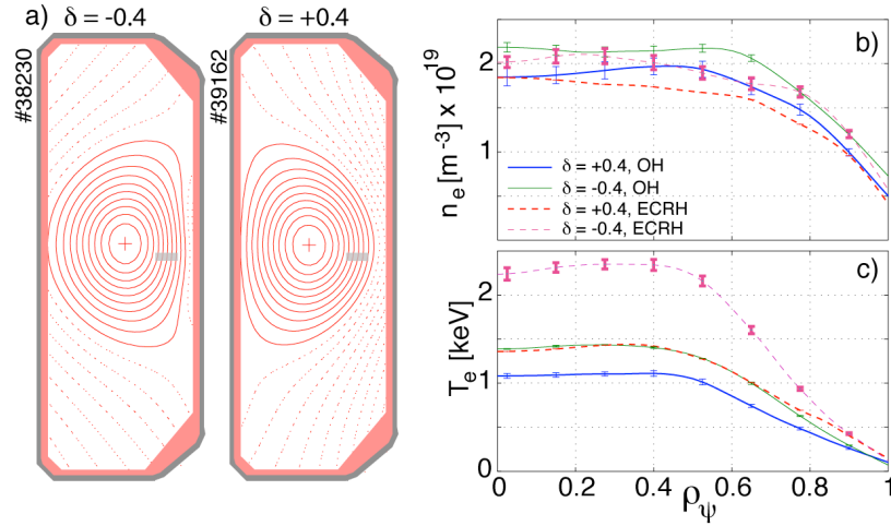
FIG. 1: a) Examples of TCV plasma shapes for negative and positive triangularity; the grey shaded area indicates the measurement location; b) density and c) temperature profiles for the four investigated cases.
