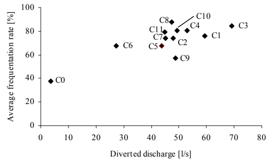
Figure 12: Average frequentionation rate of the shelter by the fishes reported to the relative diverted discharge,
