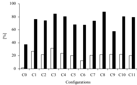
Figure 11: For configuration C0 to C11, ■ Average frequentionation rate of the shelter by the fishes, □ Diverted discharge related to hydropeaking flow.
