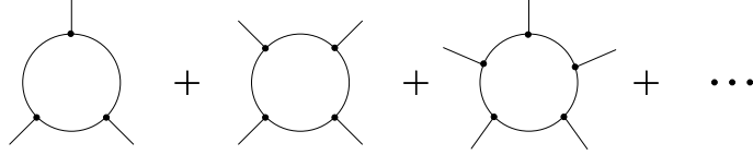
Figure 1: The graphs contributing to the 1-loop effective action, eq. (55).
