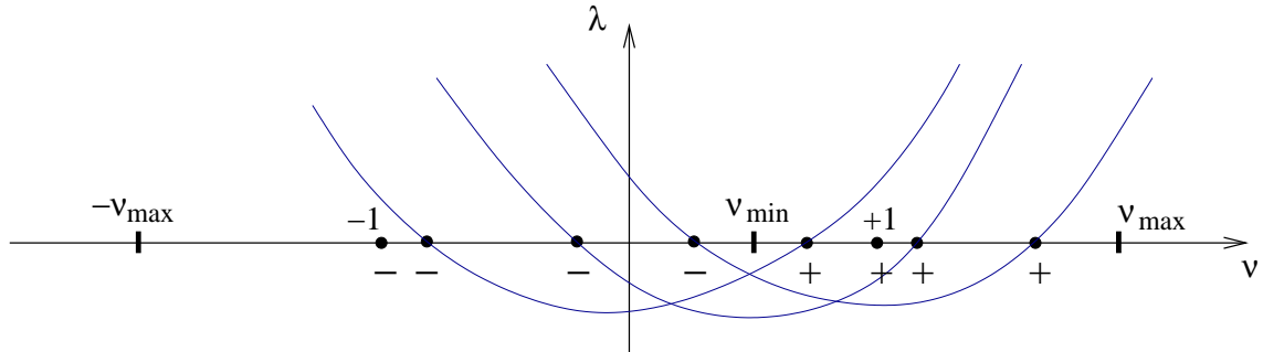
Figure 5: The eigenvalues \lambda_I of \tilde{L}_{IJ} as functions of \nu . The configuration shown corresponds to a stable system: all the positive derivative roots \nu_{I+} are on the right of the negative derivative roots \nu_{I-} (taking into account also the roots \pm 1 corresponding to the dispersion relation of the graviton). As clear from the picture, this property is equivalent to conditions (i), (ii).
