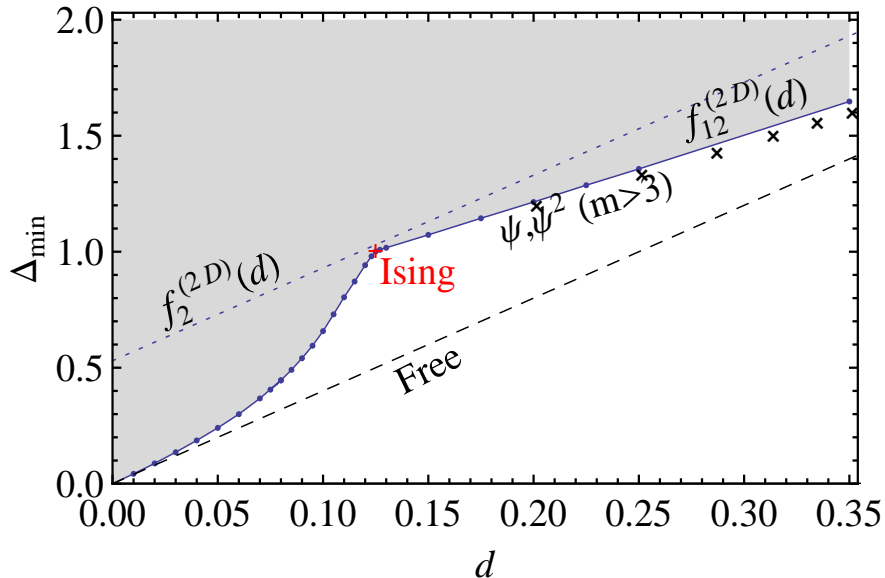
Figure 8: See the text for an explanation. The red cross denotes the position of the Ising model, the black crosses marked \psi, \psi^2 correspond to the OPEs realized in the higher minimal models, as in Fig. 15 of [7]. The shaded region is excluded.
