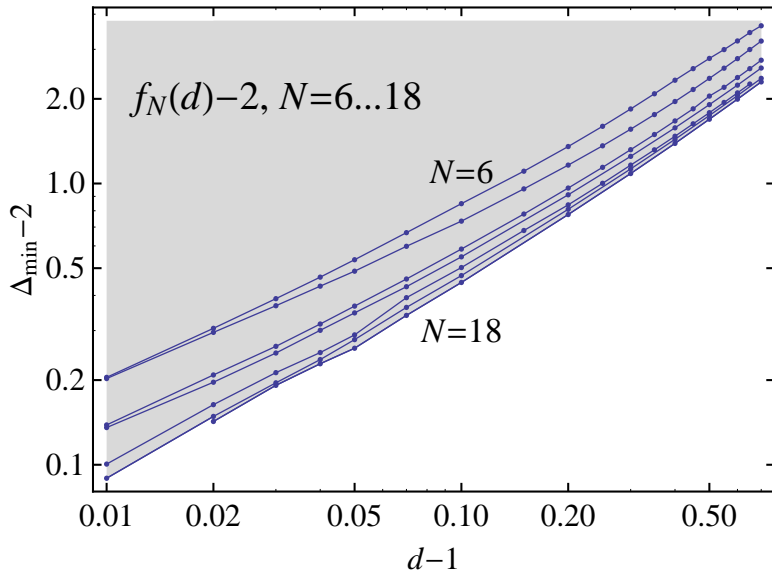
Figure 7: Same as Fig. 6 but with anomalous dimensions d - 1 , \Delta - 2 in logarithmic scale. The shaded region is excluded.
