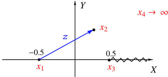
Figure 5: The auxiliary z coordinate. The conformal blocks are regular outside the cut denoted by the zigzag line.
