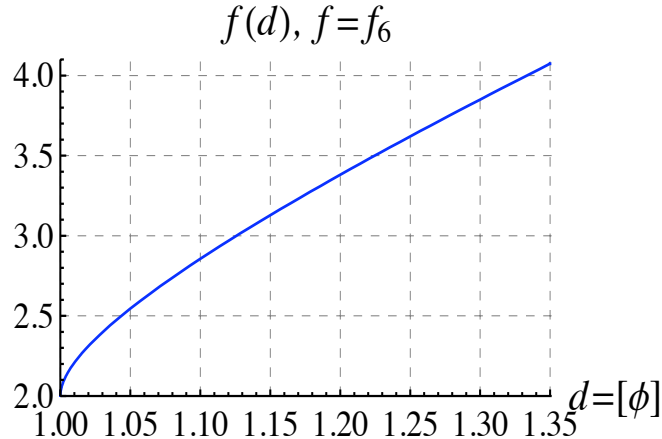
Figure 3: The bound f_6(d) \simeq 2 + 1.79\sqrt{d-1} + 2.9(d-1) , 1 \leq d \leq 1.35 , corresponding to N = 6 , reproduced from [7].
