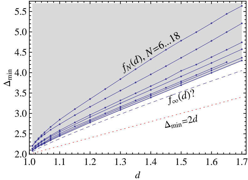
Figure 6: Our main results. The solid curves are the bounds f_N(d) , N = 6 \dots 18 . The bounds get stronger as N increases, thus N = 6 is the weakest bound (highest curve), and N = 18 is the current best bound (lowest curve). The shaded region is thus excluded. The dashed curve f_\infty(d) is an approximation to the best possible bound, obtained by extrapolating N \rightarrow \infty . The dotted line \Delta_{\min} = 2d is realized in a family of “generalized free scalar” CFTs, and is compatible with our bounds.
