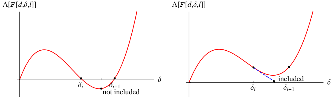
Figure 9: Imposing the positivity of the functional on a discrete set of points, it could happens that the intermediate points don't satisfy \Lambda[\mathcal{F}[d, \delta, l]] \geq 0 (on the left). However adding the constraint \Lambda[\mathcal{F}_{1/2}[d, \delta_i, l]] \geq 0 , see (A.9), we can be sure that the functional is positive on all the neglected points (on the right).
