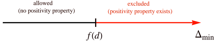
Figure 2: The bound f(d) is the smallest \Delta_{\min} for which a positivity property exists.
