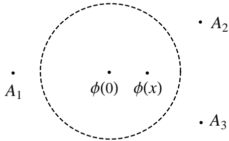
Figure 4: The operator product expansion of \phi(x)\phi(0) converges for this configuration.
