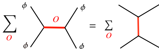
Figure 1: The conformal bootstrap equation. The thick red line denotes a conformal block, summing up exchanges of a primary operator O and all its descendants.
