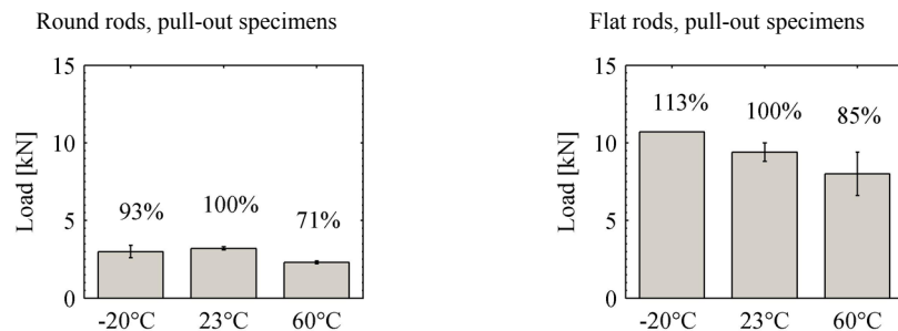
Figure 5: Bar graph of the mean pull-out strength values relative to the reference temperature 23^{\circ}\text{C} .
