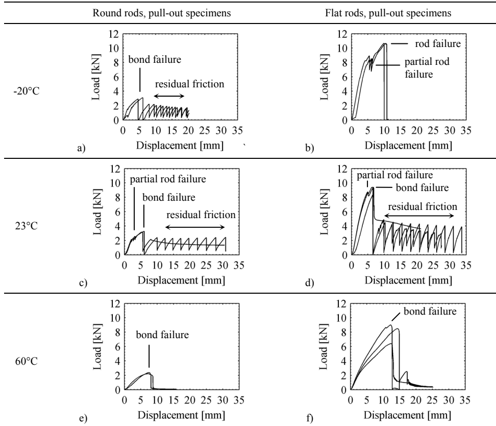
Figure 3: Load-displacement diagrams of the pull-out tests.
