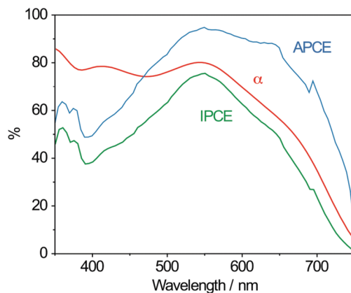
FIGURE 3. Absorbance spectrum ( \alpha ) calculated from measured diffuse reflectance ( R_d ) and diffuse transmittance ( T_d ) spectra of a C101 dye-sensitized, 6 \mu\text{m} thick film made of \text{TiO}_2 fibers. The IPCE photocurrent action spectrum was recorded for DSCs based on similar dye-sensitized 6 \mu\text{m} thick films. The absorbed photon-to-current conversion efficiency (APCE = IPCE/ \alpha ) data were finally extracted from the two latter spectra.
