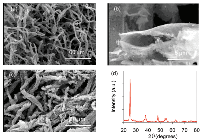
FIGURE 2. (a) SEM micrograph of \text{TiO}_2 fibers just after the organic template was removed by heat treatment. (b) SEM image showing the cross section of one hollow fiber. (c) Typical SEM image of \text{TiO}_2 nanofibers obtained after milling and ultrasonication to make a paste. (d) XRD diagrams of the \text{TiO}_2 fibers.
