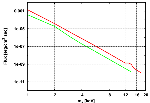
Figure 3. Comparison between Coma center (red curve) and Coma 3 (green curve) fluxes (per 200 eV energy bin).
