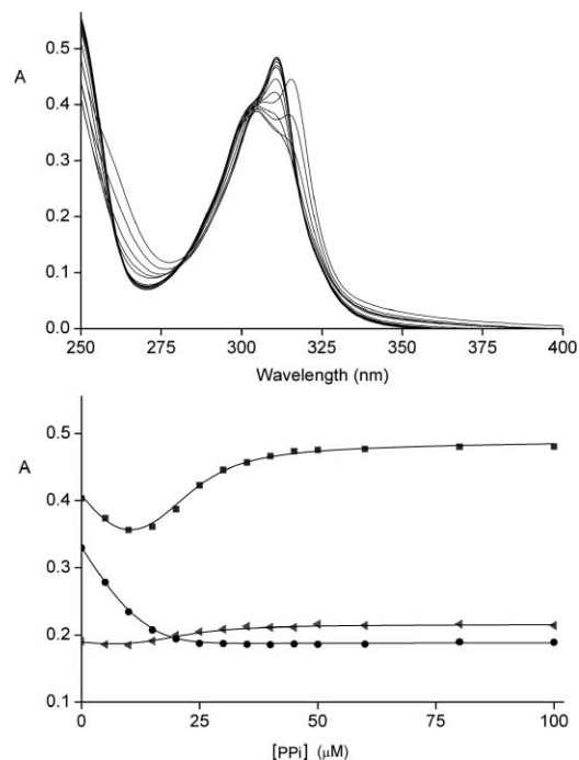
Fig. 1 Top: absorption spectra of solutions containing the palladium complex 1 (25 μM) and different amounts of PPi (0–100 μM). The spectra were recorded in aqueous HEPES buffer solution (25 mM, pH 7.0) after equilibration. Bottom: variation in absorbance at λ = 290 (▲), 310 (■) and 320 nm (●). The lines represent the best fit to the model discussed in the main text.
