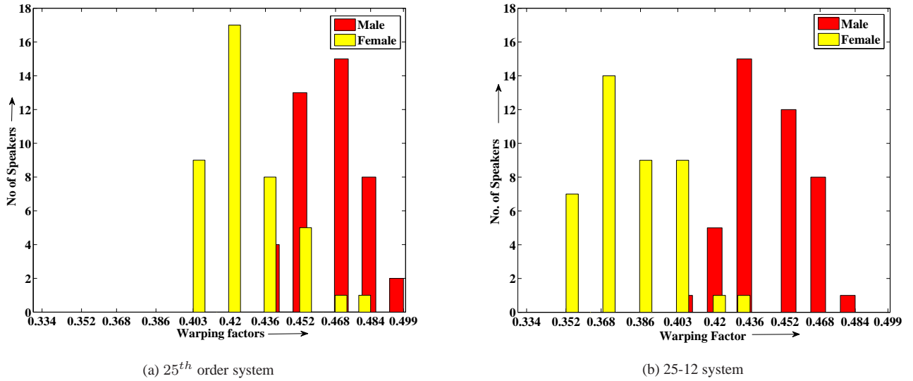
Fig. 2: Warping factors estimated from 25 th order features. The 25-12 system initializes the features with the warping factors estimated from 12 th order features. Both graphs have same range for X-axis.
