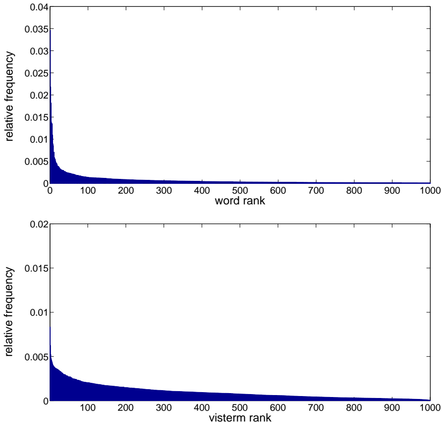
Fig. 2. Top: relative frequency distribution of the words extracted from REUTERS-21578, first 1000 words. Bottom: relative frequency distribution of the visterms in the city-landscape data set D1 .
