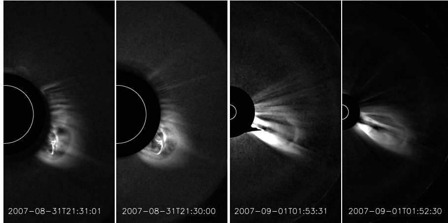
Fig. 1. The CME on 31 August - 1 September 2007 observed by SECCHI-COR1 (the left two columns) and by SECCHI-COR2 (the right two columns) coronagraphs. Both A (second and fourth columns) and B (first and third columns) spacecraft images are shown. COR1 images show the white light total brightness corona from 1.4 to 4 R_{\odot} . COR2 images show the white light total brightness corona from 2.5 to 15 R_{\odot} . In all panels the visible solar disc is represented by the white circle, while the larger dark disc shows the coronagraph occulter. The images were co-aligned in the STEREO mission plane. Adapted from Mierla et al. (2009).
