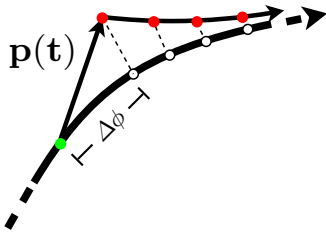
Fig. 3 Effect of a small pulse like perturbation on the limit cycle. The perturbation \mathbf{p}(t) arrives when the phase point is at the position marked by a the green dot. The phase point is then pushed back to the limit cycle by the stability properties of the system, i.e. it approaches asymptotically the limit cycle. It however retains a phase difference ( \Delta\phi ) in comparison with the unperturbed reference system. The phase difference can be of different amplitude and sign depending on the direction of the perturbation and the state the system currently is in when the perturbation arrives. Understanding this fact is key to understanding synchronization phenomena.
