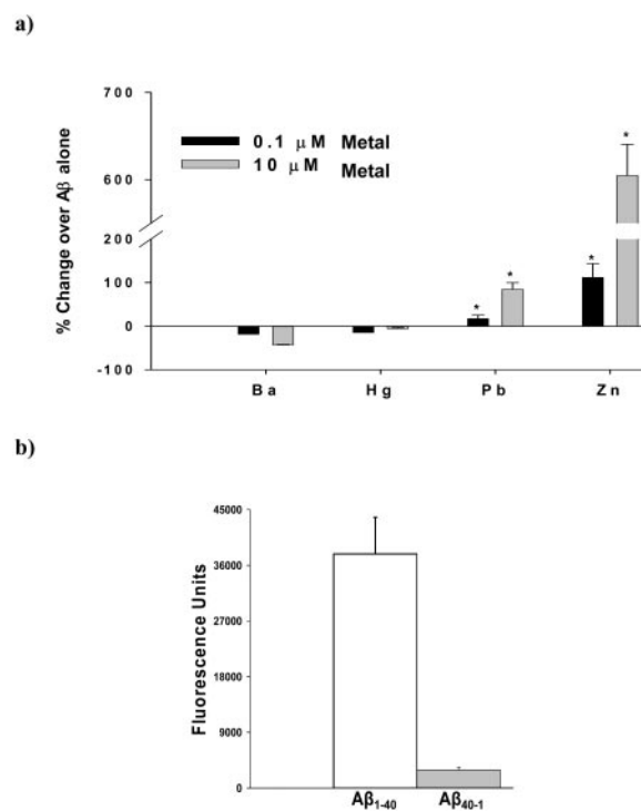
Figure 1. Fluorimetric detection of A \beta 1-40 aggregation and its reverse sequence peptide A \beta 40-1 (control) using bis-ANS. a) A \beta 1-40 samples were prepared for the fluorescence studies and the emission spectra was recorded at 455–550 nm. The intensity of fluorescence was used as a measure of aggregation. Values shown are the mean \pm SE ( n=4 ). *Significantly different from control ( P<0.05 ) as determined by ANOVA and Duncan's post hoc test. b) Affinity of bis-ANS to bind A \beta 1-40 and A \beta 40-1 (control peptide).
