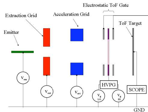
Figure 3. Schematic of TOF configuration for EPFL emitters.
