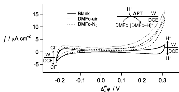
Figure 2. Cyclic voltammograms obtained with the electrochemical cell shown in Figure 1 in the absence of DMFc (—, aerobic) and in the presence of DMFc (•••••, aerobic; ----, anaerobic); scan rate 0.05 \text{ Vs}^{-1} . APT = assisted proton transfer.
