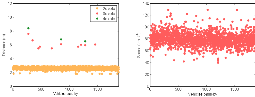
Figure 5. Distance between axles (left), and speed (right) for vehicle pass-by of category 1
