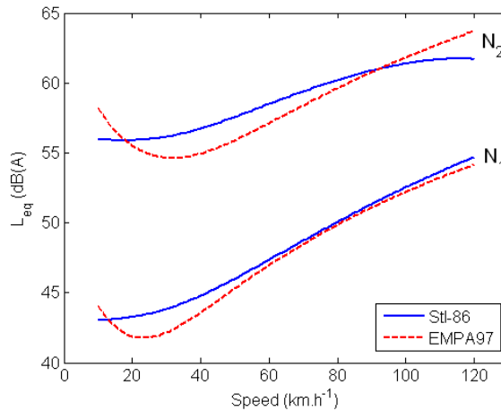
Figure 1. Comparison between StL86+ and EMPA97 noise levels for N_1 and N_2 categories
