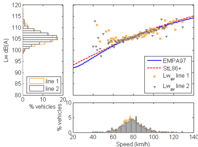
Figure 6. Speed versus average emission level (center), vehicles distribution versus emission level (left) and vehicles distribution versus speed (bottom) for EUR13 C1 category
