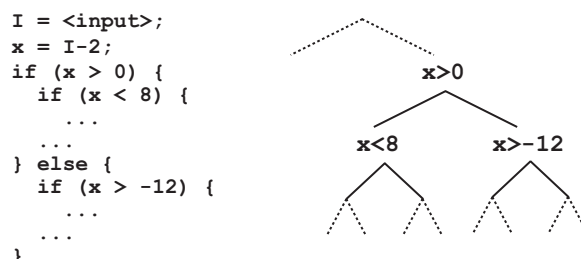
Figure 1. A program and its symbolic execution tree.
